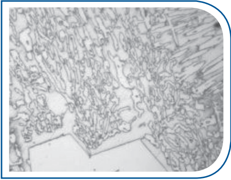
D60 microstructure at 1000x magnification
