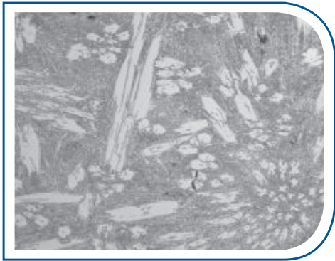
D60 microstructure at 100x magnification
